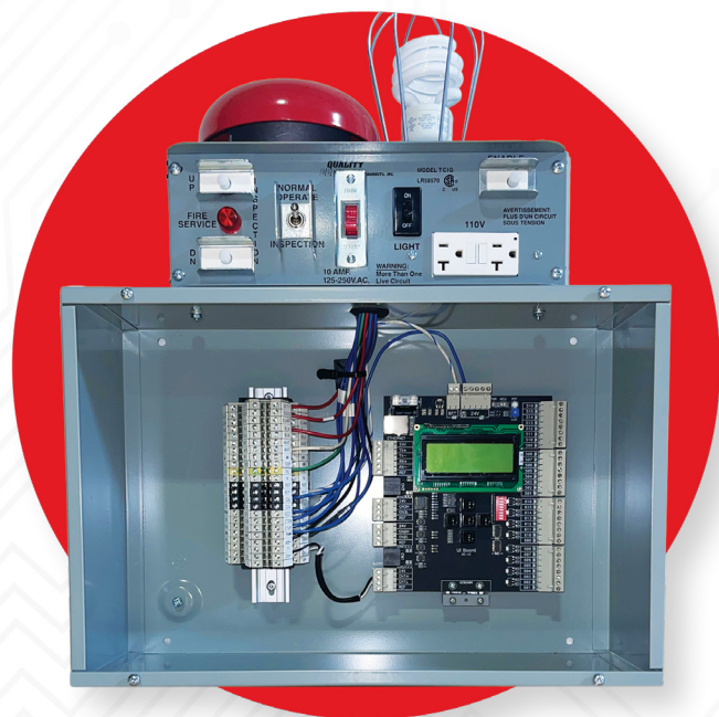
Car Top with Pre-Wired Inspection Station
